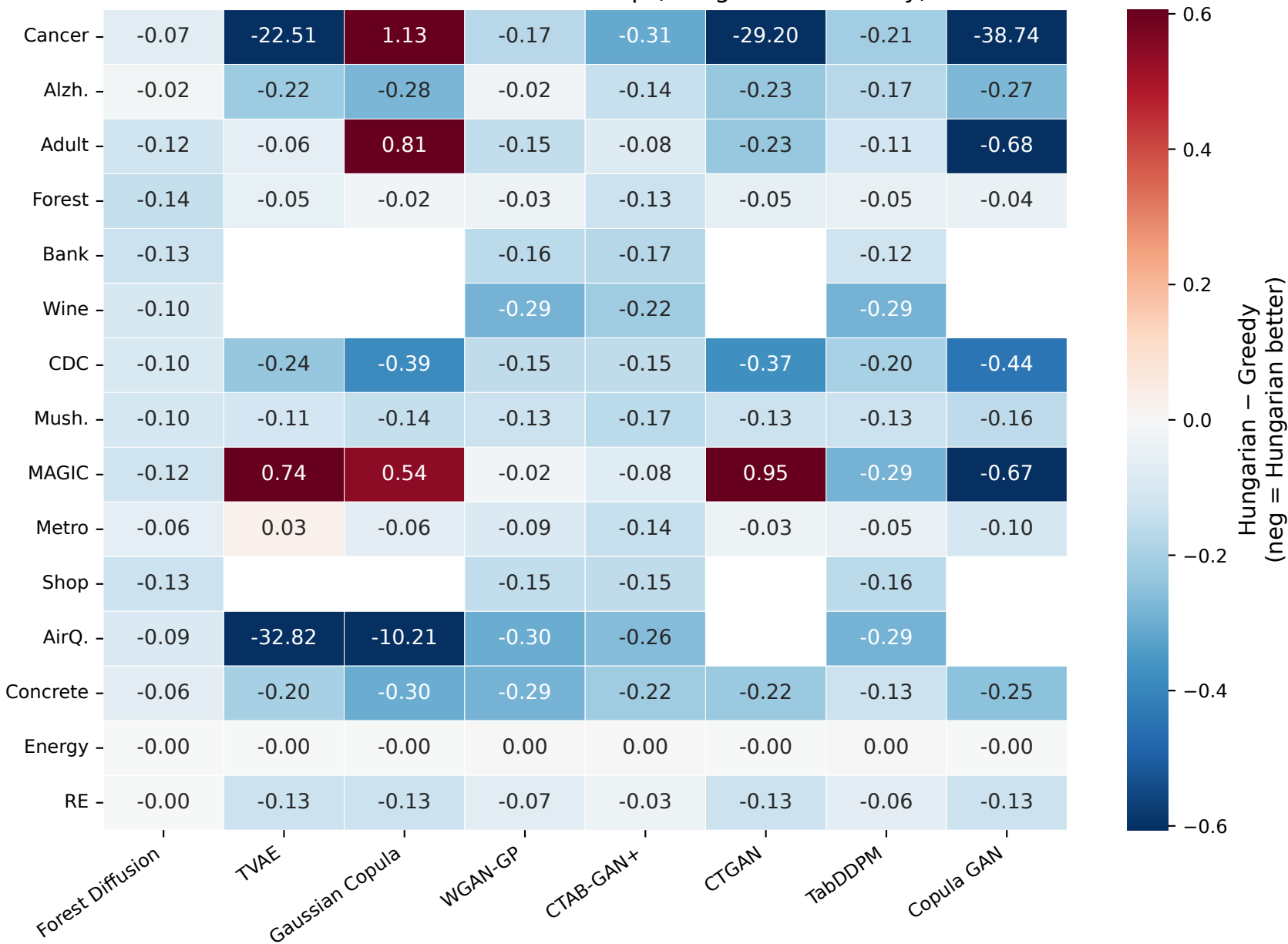
Mahalanobis difference heatmap (Hungarian – Greedy)
